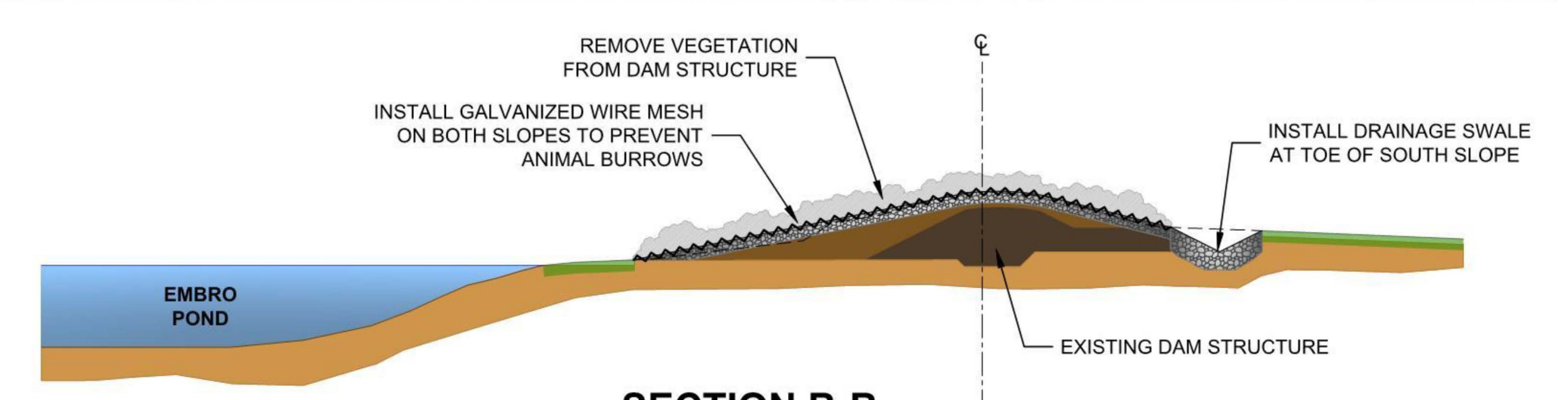
SECTION B-B
