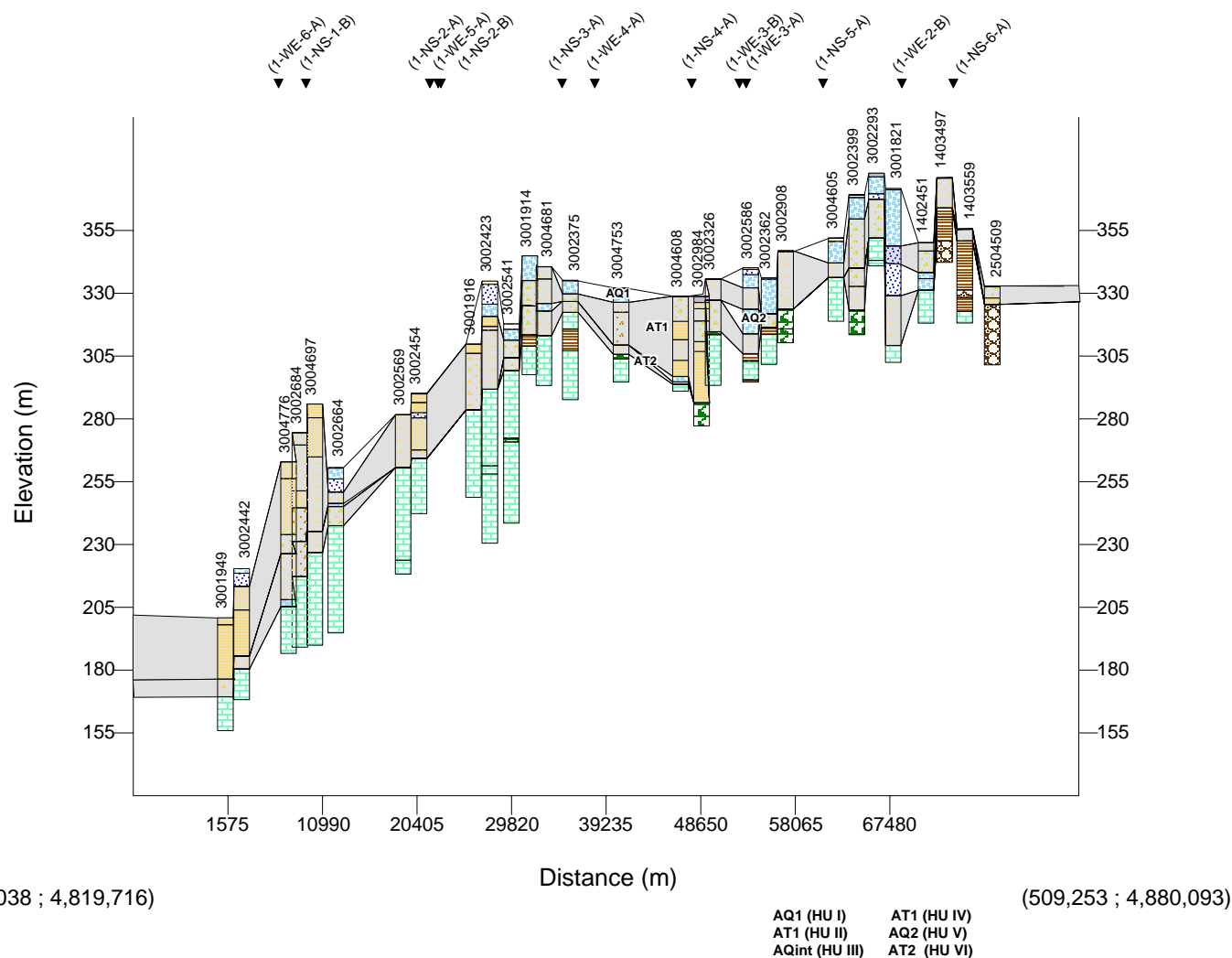
Figure 1-5: Regional Cross-section A-A'
