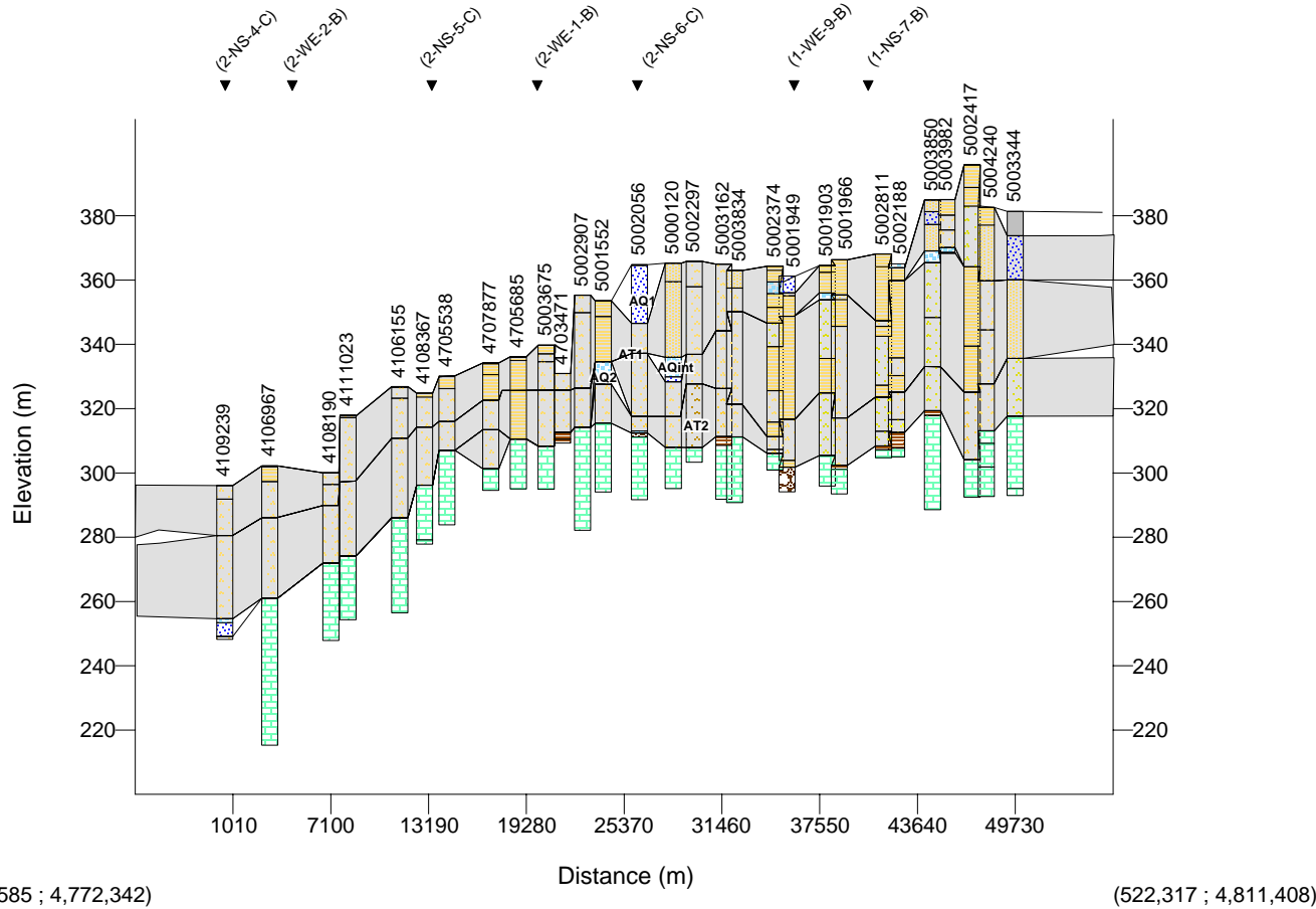
Regional Cross-section F-F' Vertical Exaggeration: 200
