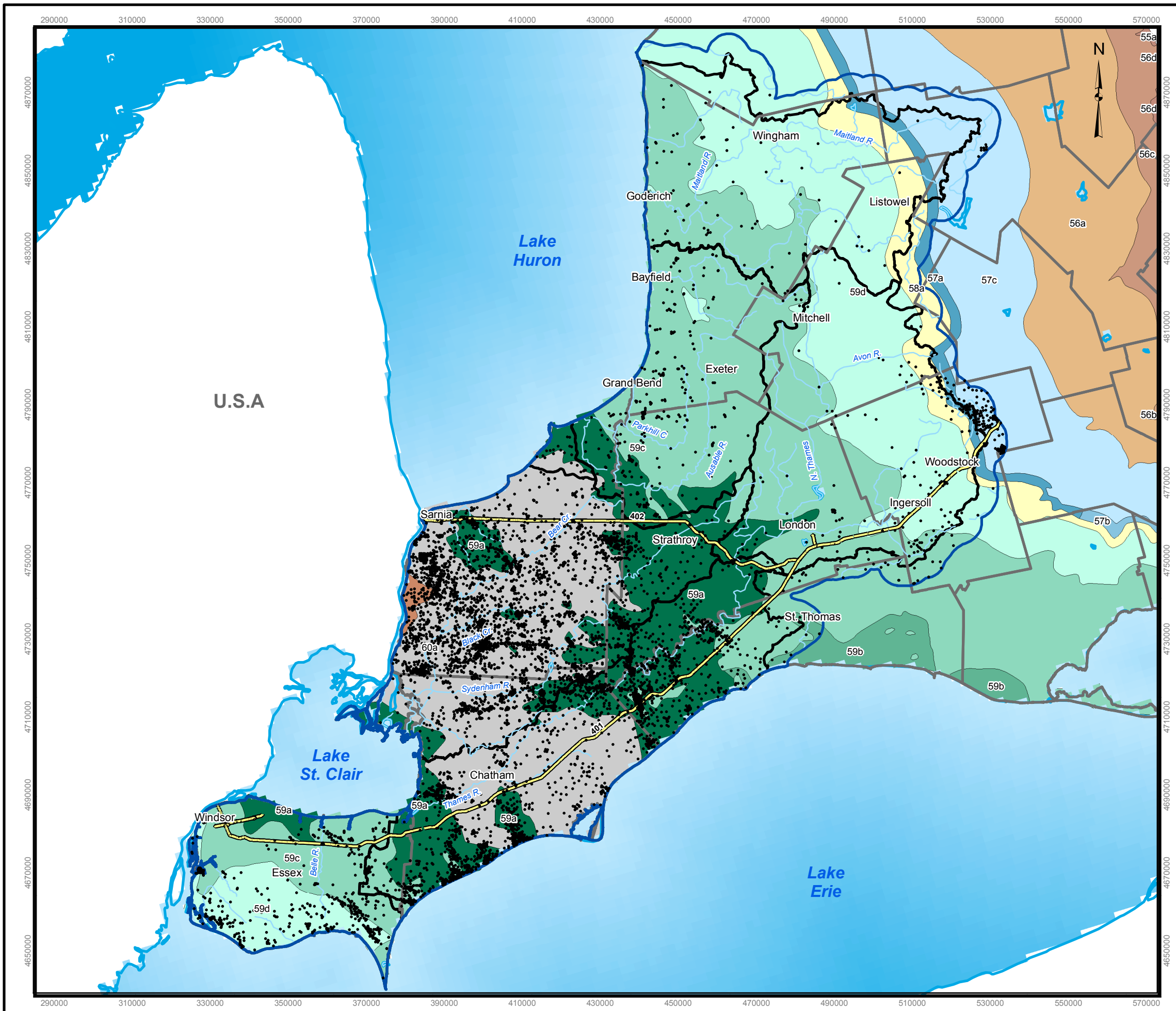
Figure 13: Bedrock Geology
