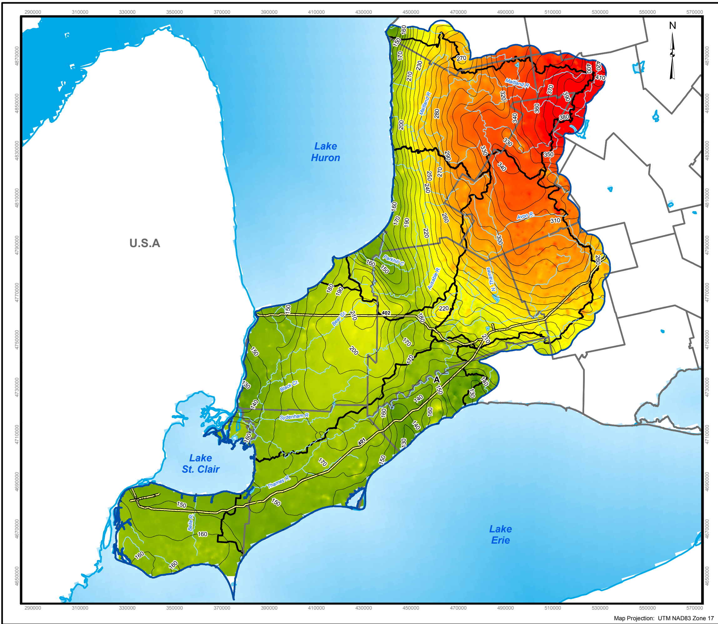
Figure 14: Bedrock Topography
