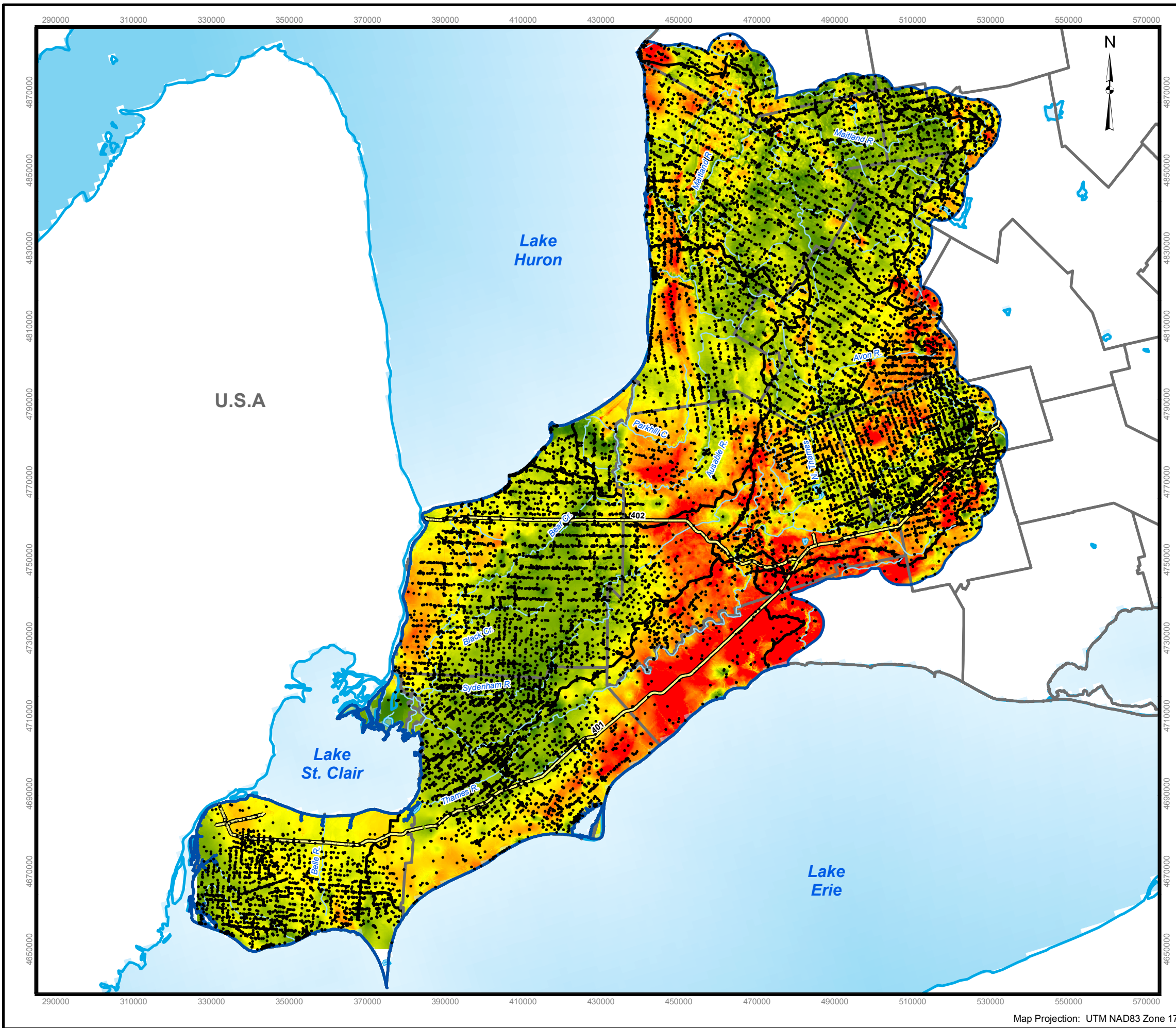
Figure 15: Overburden Thickness
