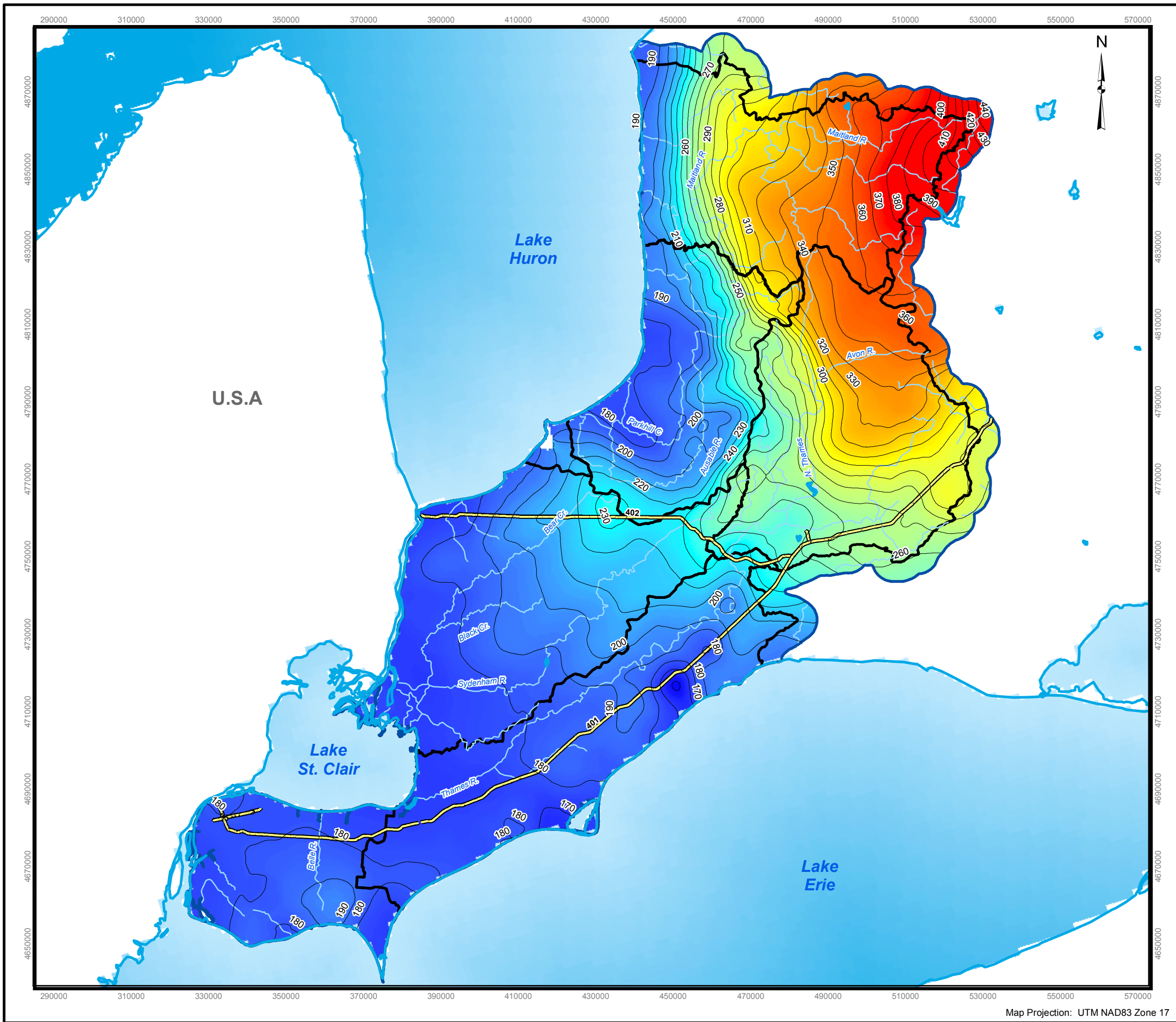
Figure 2-8: Observed Bedrock Equipotentials
