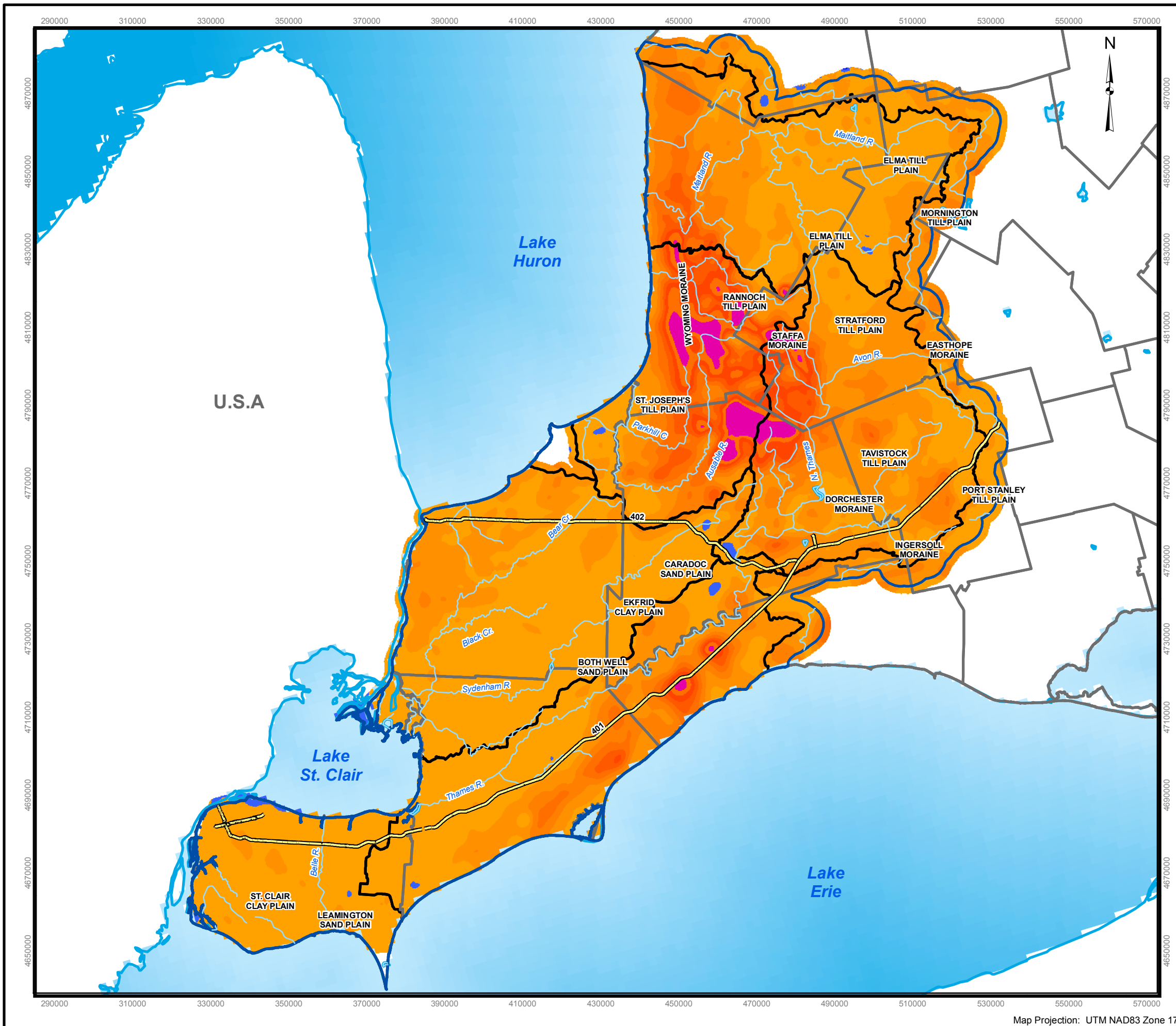
Figure 2-10: Estimated Zones of Potential Recharge and Discharge Areas
