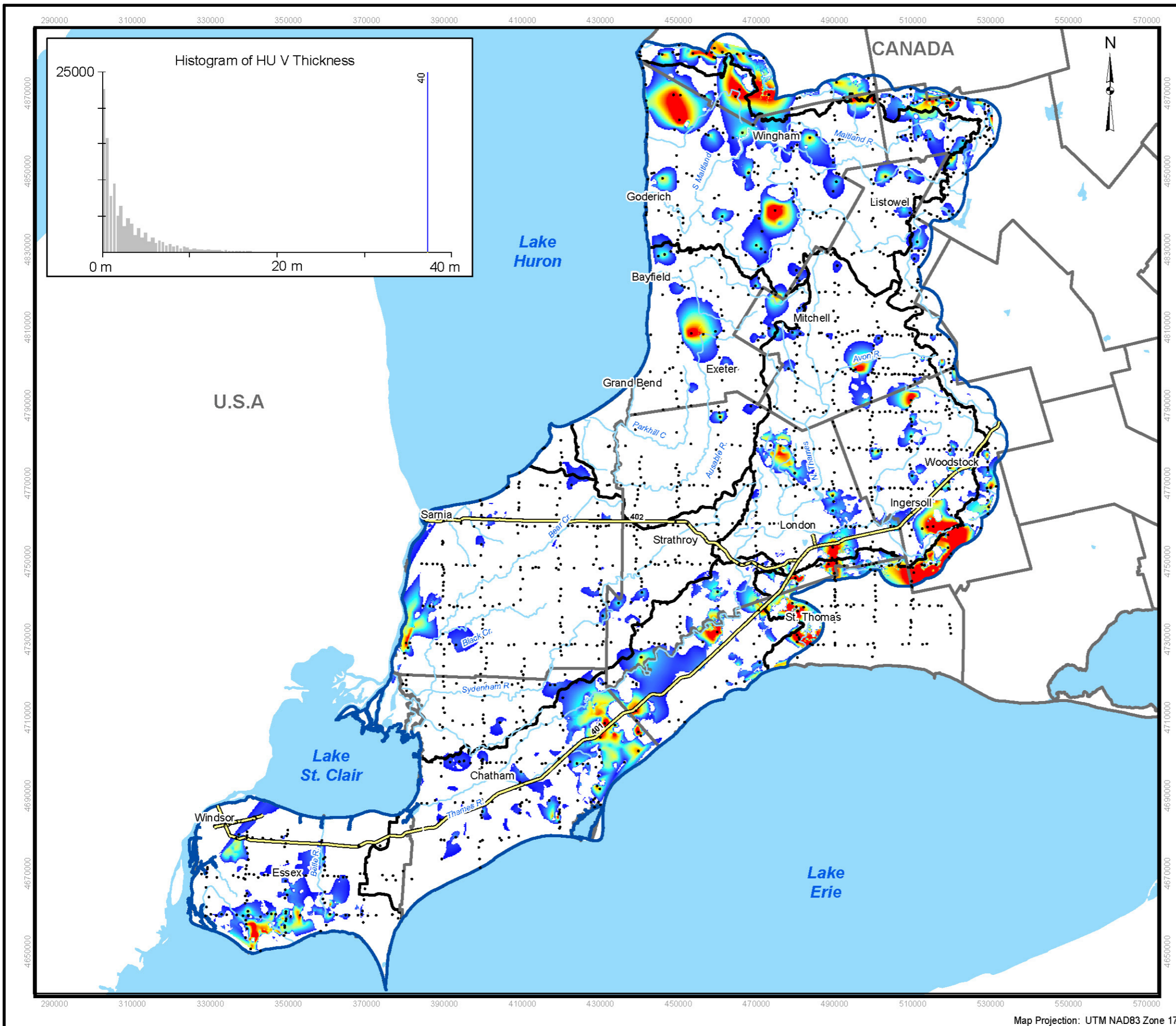
Figure 21: Isopach Aquifer HU V (AQ2)
