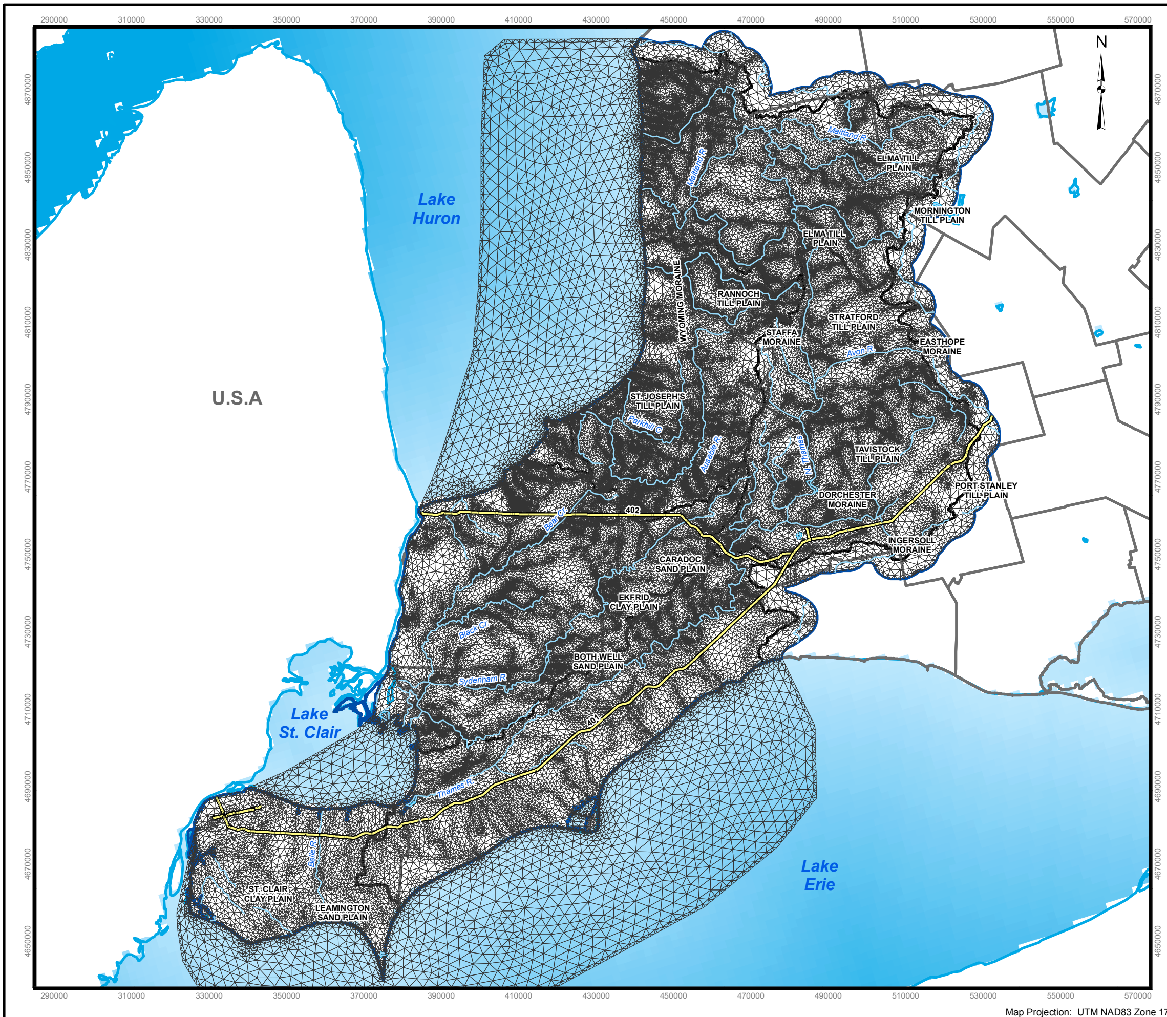
Figure 4-1: FEFLOW Finite Element Mesh
