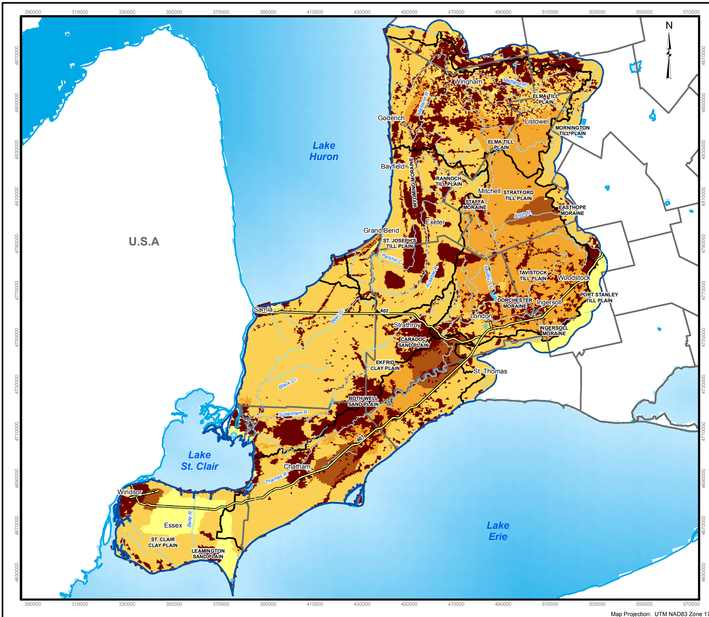
Figure 4-17: Recharge Distribution - Model Layer 1
