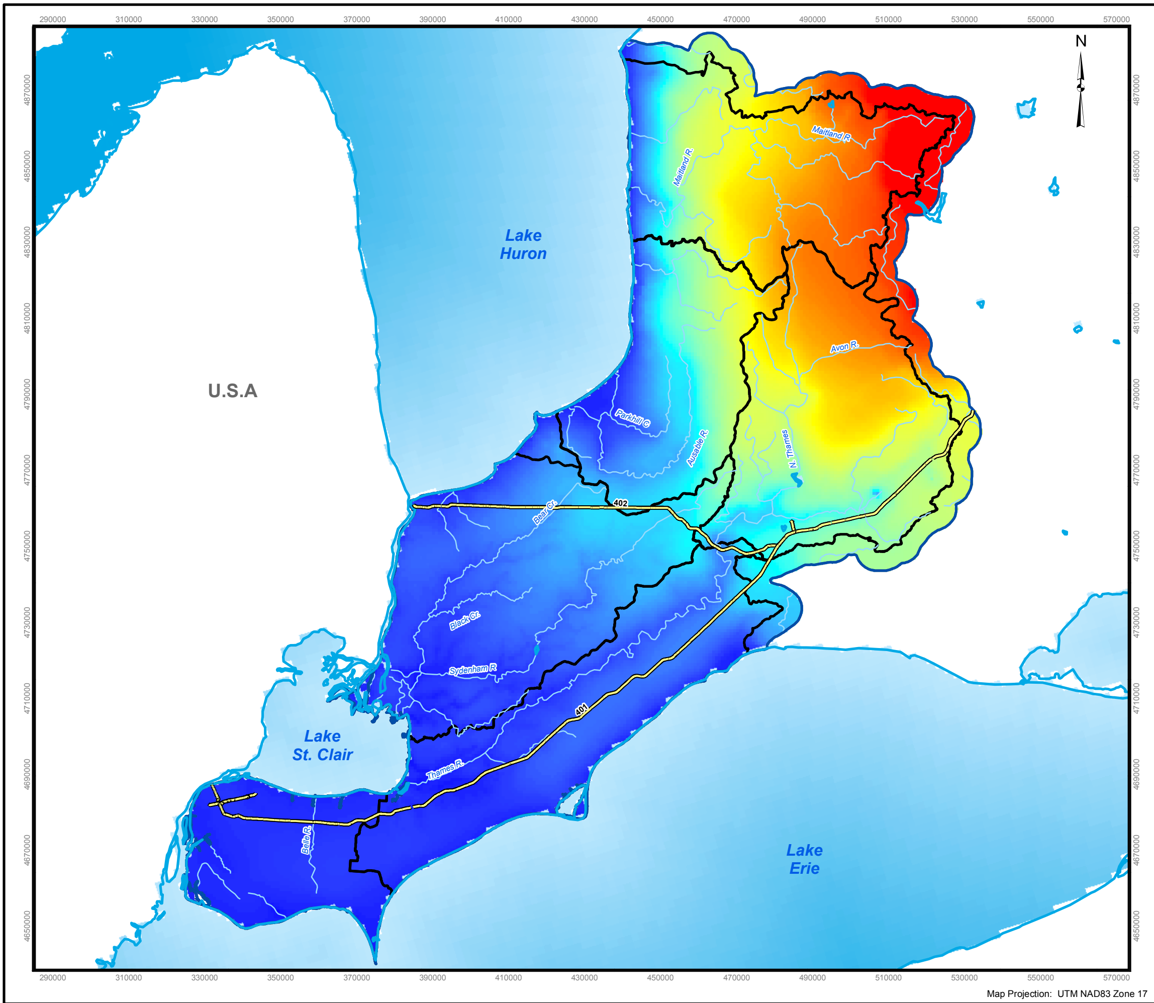
Figure 5-3: Modeled Bedrock Potentiometric Surface
