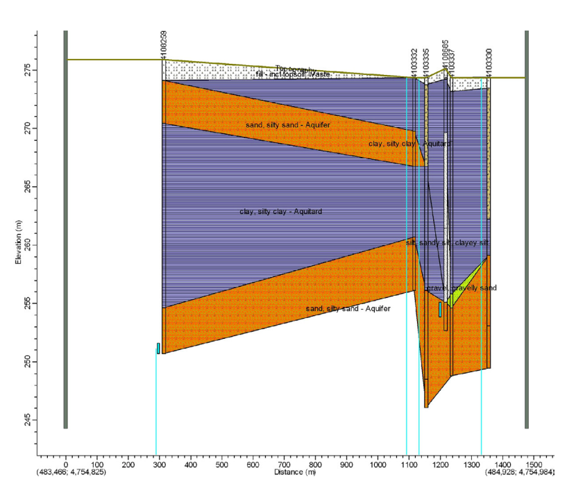
Cross Section: WM1 - WM1'
