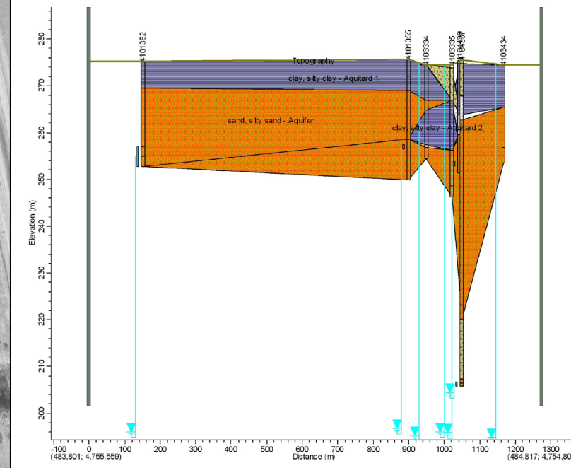
Cross Section: WM2 - WM2'
